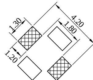
( PCB Pattern )
